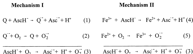
Fig. 2. Two mechanisms of redox cycling of VC and VK 3 .
