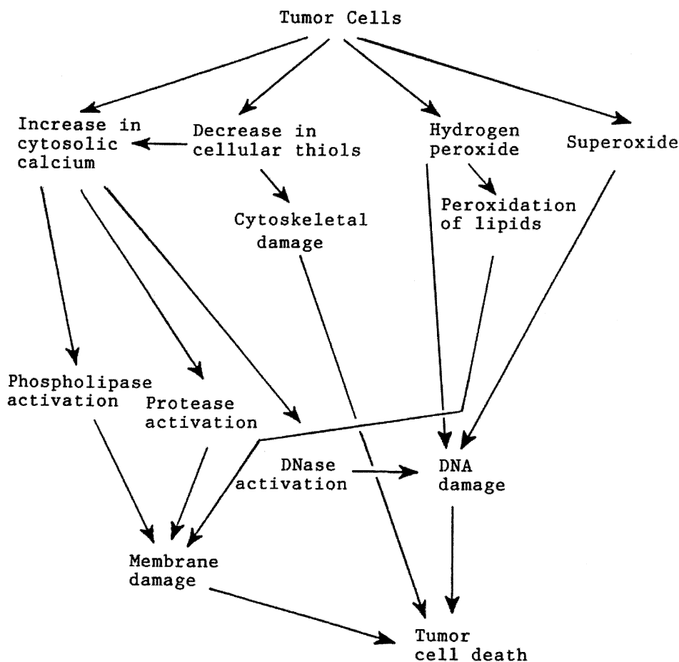
Fig. 4. A schematic of the mechanisms by which VC/VK 3 induce autoschizis.
